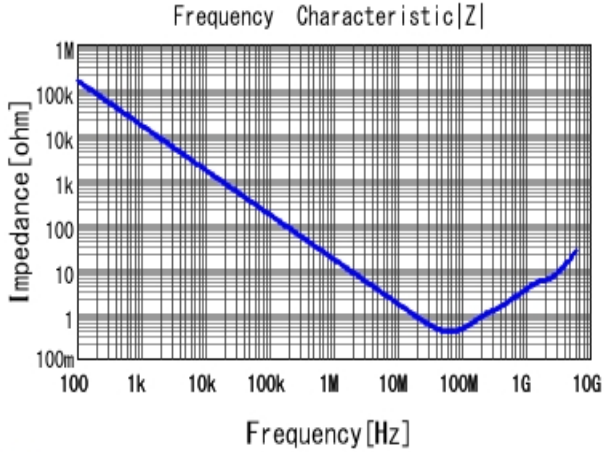
■ GCJ216R72A103KA01 |Z| DC0V, 25degC
