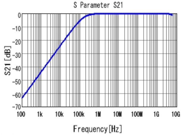
■ GCJ216R72A103KA01 S21 DC0V, 25degC
