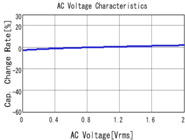
■ GCJ216R72A103KA01 C-AC Voltage capchange, DC0V, 25.0d
