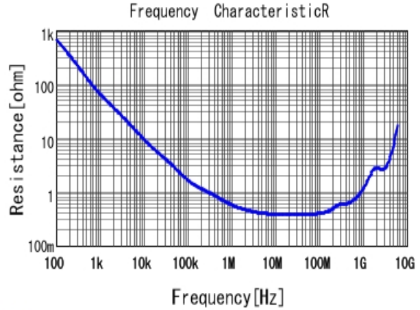
■ GCJ216R72A103KA01 R DC0V, 25degC
