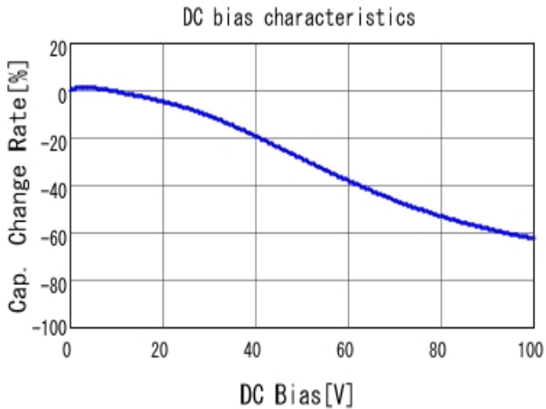
■ GCJ216R72A103KA01 C-DC bias capchange, 25.0degC, AC1.
