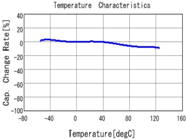
■ GCJ216R72A103KA01 C-Temp. capchange, DC0.0V, AC1.0Vrm
