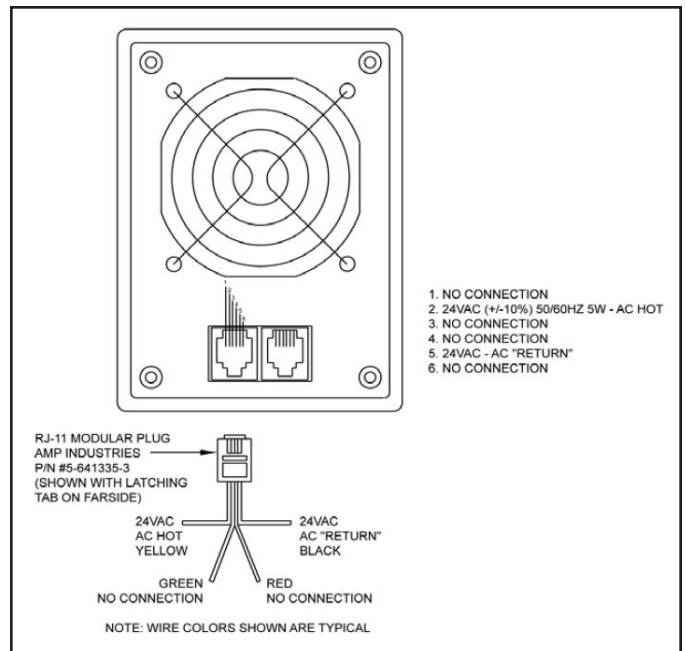
Figure 3. Pin-out of RJ11 power plug and inlet
