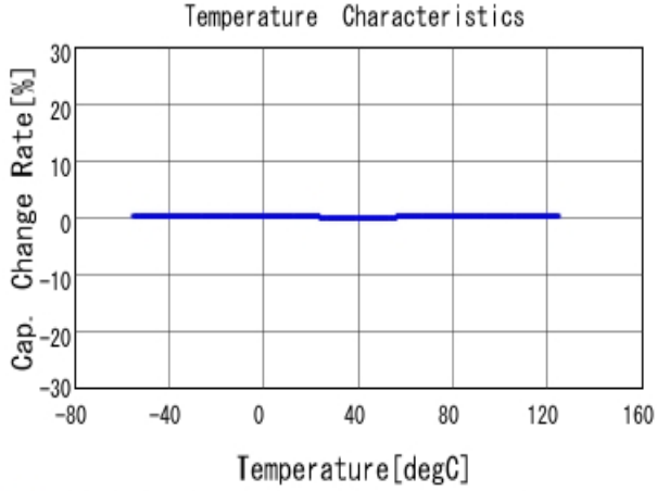
■ GRM1555C1H6R8DA01 C-Temp. capchange, DCOV, AC1Vrms
