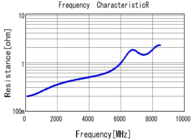
■ GRM1555C1H6R8DA01 R DCOV, 25degC
