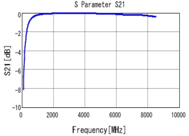
■ GRM1555C1H6R8DA01 S21 DCOV, 25degC
