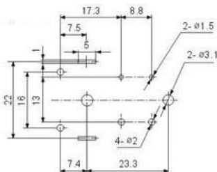
Mounting
