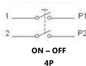
Circuitry
