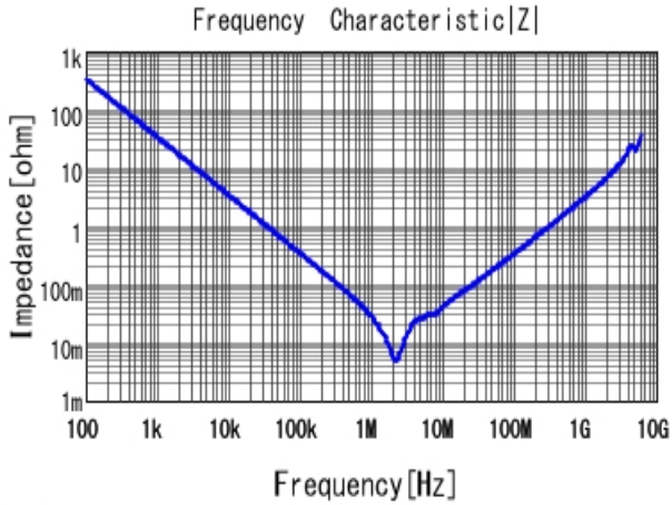
■ GRM31CR61A475KA01 |Z| DCOV, 25degC
