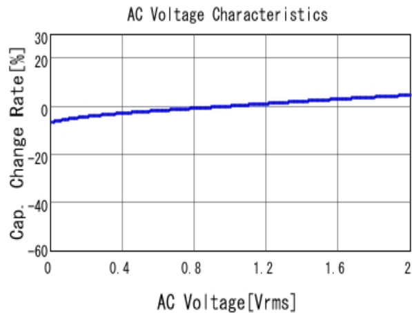
■ GRM31CR61A475KA01 C-AC Voltage capchange, DCOV, 25.0d
