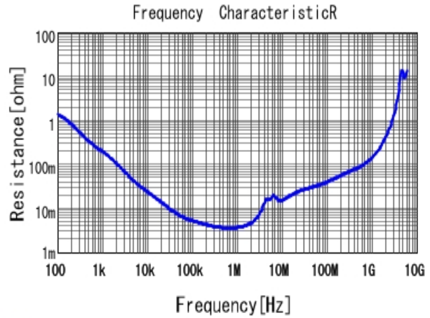
■ GRM31CR61A475KA01 R DCOV, 25degC
