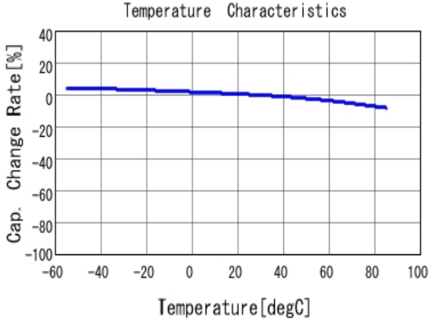
■ GRM31CR61A475KA01 C-Temp. capchange, DC0.0V, AC1.0V r m
