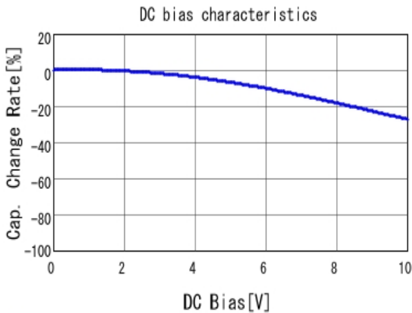
■ GRM31CR61A475KA01 C-DC bias capchange, 25.0degC, AC1.
