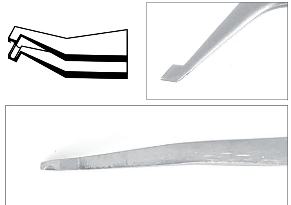
SM111.SA 4 3/4" 120 mm For holding and positioning 0.5-1 mm cylindrical devices; flat base grooved tips ( 2 mm long)
