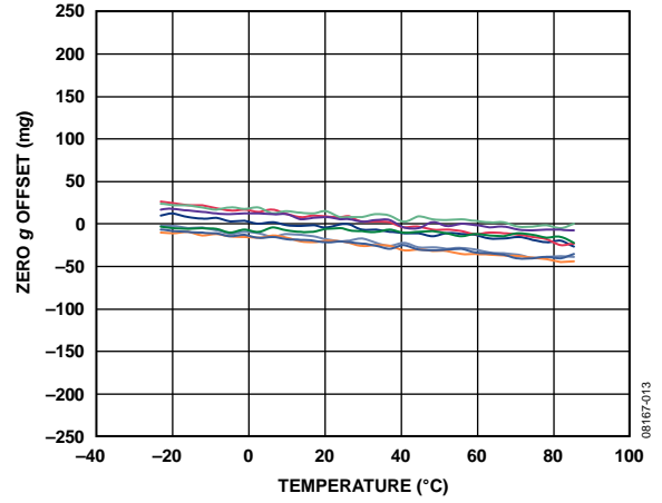
Figure 13. X-Axis Zero g Offset vs. Temperature— Eight Parts Soldered to PCB, V_S = 2.6 V
