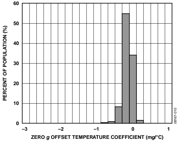
Figure 10. X-Axis Zero g Offset Temperature Coefficient, V_S = 2.6 V
