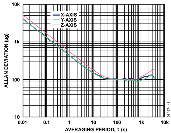
Figure 55. Allan Deviation
