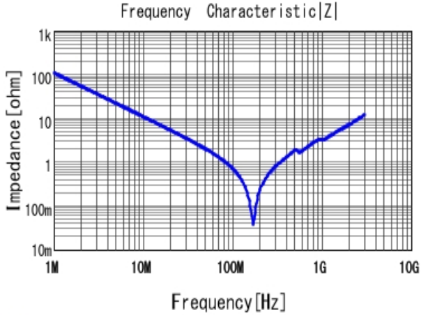
■ GRM32A7U2J152JW31 |Z| DCOV, 25degC
