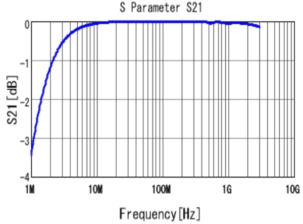
■ GRM32A7U2J152JW31 S21 DCOV, 25degC
