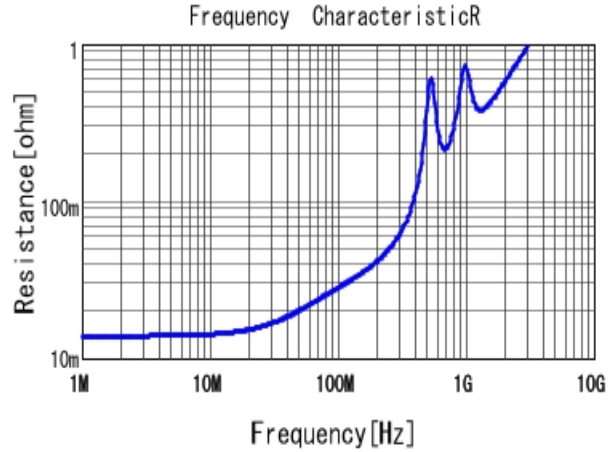
■ GRM32A7U2J152JW31 R DCOV, 25degC
