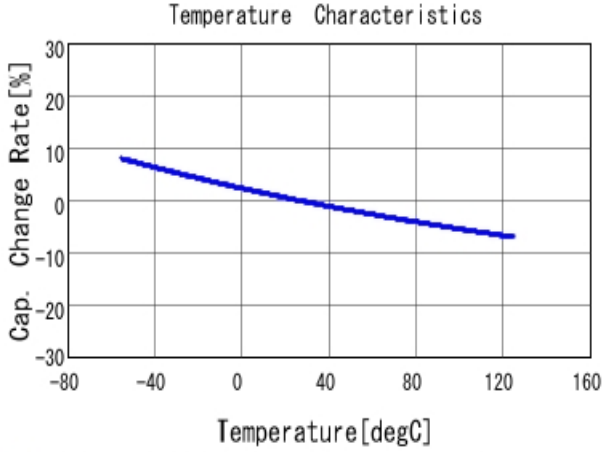
■ GRM32A7U2J152JW31 C-Temp. capchange, DCOV, AC1Vrms
