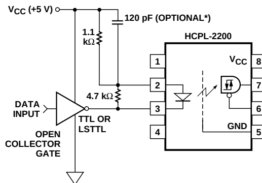
Figure 16. Series LED Drive with Open Collector Gate (4.7 k \Omega Resistor Shunts I_{OH} from the LED).
