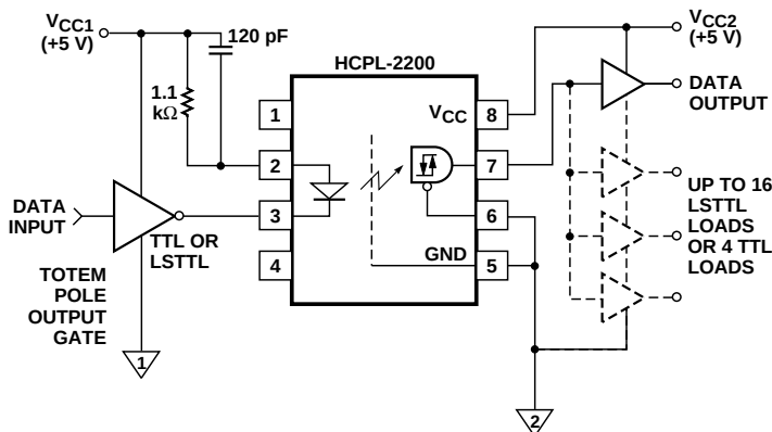
Figure 13. Recommended LSTTL to LSTTL Circuit.
