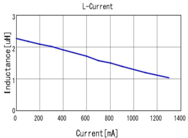
■ LQM31PN2R2M00 L-Current 20degC
