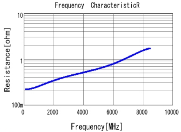
■ GRM0335C1H4R7CA01 R DC0V, 25degC
