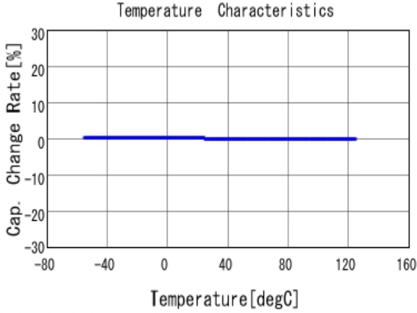
■ GRM0335C1H4R7CA01 C-Temp. capchange, DCOV, AC1Vrms
