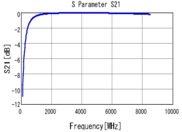
■ GRM0335C1H4R7CA01 S21 DCOV, 25degC
