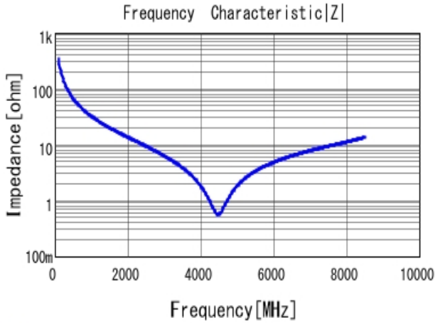
■ GRM0335C1H4R7CA01 |Z| DC0V, 25degC
