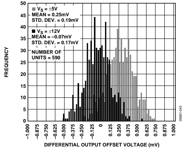
Figure 33. Differential Output Offset Voltage Distribution
