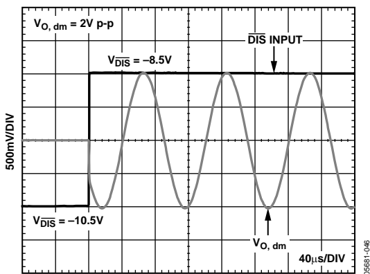
Figure 36. Disable Turn-On Time
