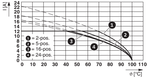
Type: MVSTBR 2,5/...-ST-5,08 with SMSTBA 2,5/...-G-5,08
