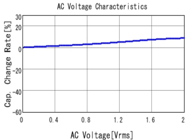
■ KRM55WR71J226MH01 C-AC Voltage capchange, DCOV, 25.0d
