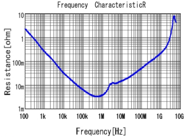
■ GRM31CR70J226ME19 R DCOV, 25degC
