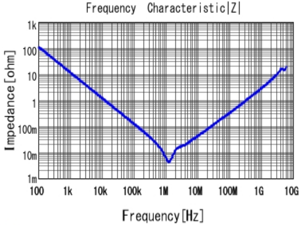
■ GRM31CR70J226ME19 |Z| DCOV, 25degC
