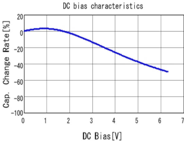
■ GRM31CR70J226ME19 C-DC bias capchange, 25.0degC, ACO.
