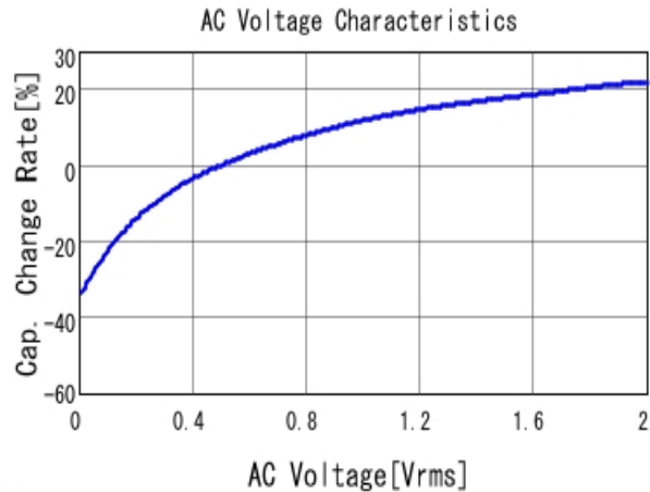
■ GRM31CR70J226ME19 C-AC Voltage capchange, DCOV, 25.0d
