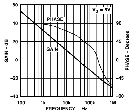
TPC 21. Open-Loop, Gain and Phase vs. Frequency
