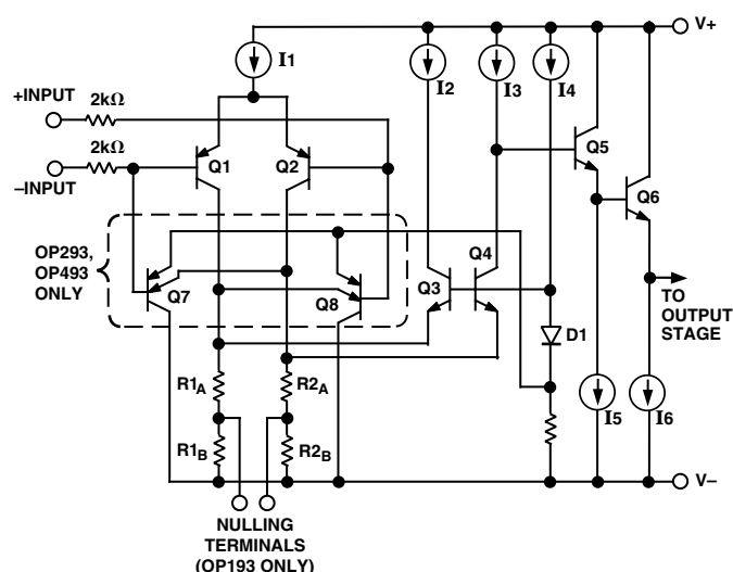
Figure 1. OP193/OP293/OP493 Equivalent Input Circuit
