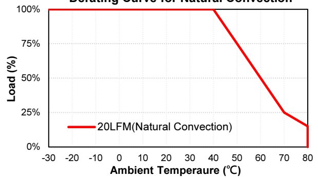
CFM81S150/240/480-CA Derating Curve for Natural Convection
