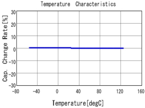
■ GCM3195C2A103JA16 C-Temp. capchange, DCOV, AC1Vrms
