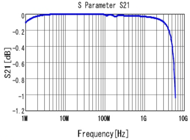
■ GCM3195C2A103JA16 S21 DCOV, 25degC
