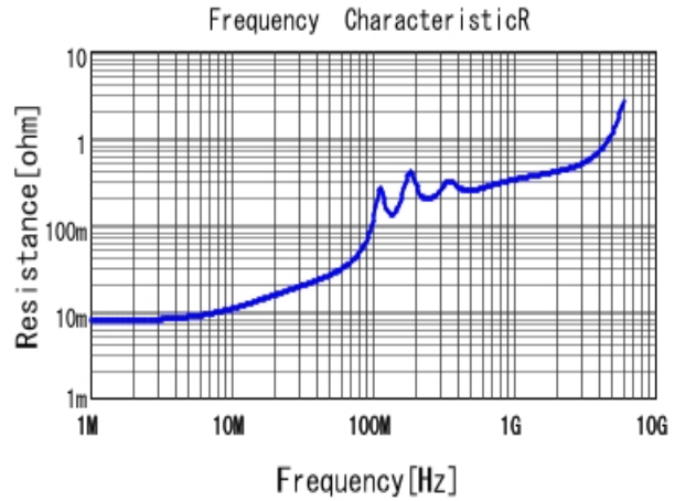
GCM3195C2A103JA16 R DCOV, 25degC
