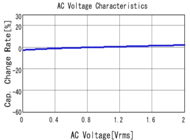
■ GRM31MR72A683KA01 C-AC Voltage capchange, DCOV, 25.0d
