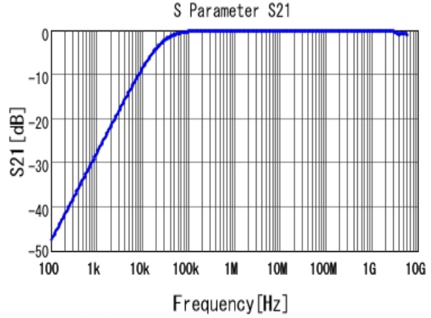
■ GRM31MR72A683KA01 S21 DCOV, 25degC
