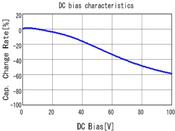
■ GRM31MR72A683KA01 C-DC bias capchange, 25.0degC, AC1.
