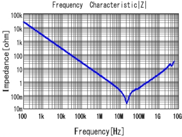
■ GRM31MR72A683KA01 |Z| DCOV, 25degC
