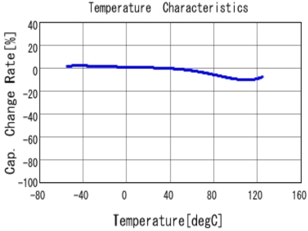
■ GRM31MR72A683KA01 C-Temp. capchange, DCO. 0V, AC1.0V rm
