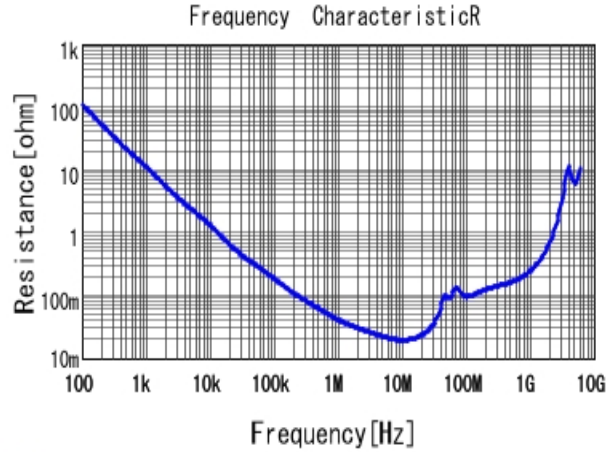
■ GRM31MR72A683KA01 R DCOV, 25degC
