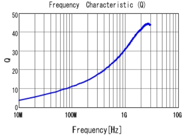
■ LQG15HS3N9S02 Q
