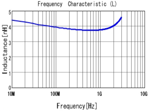
■ LQG15HS3N9S02 L
