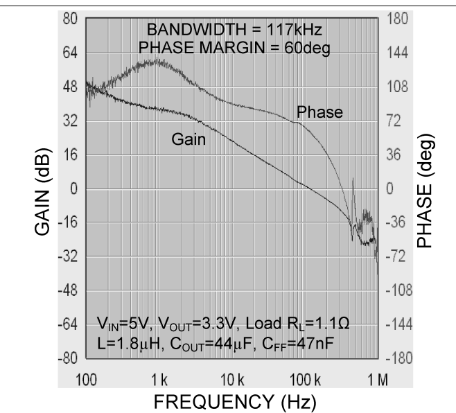
Figure 23. Loop Gain and Phase With C FF
