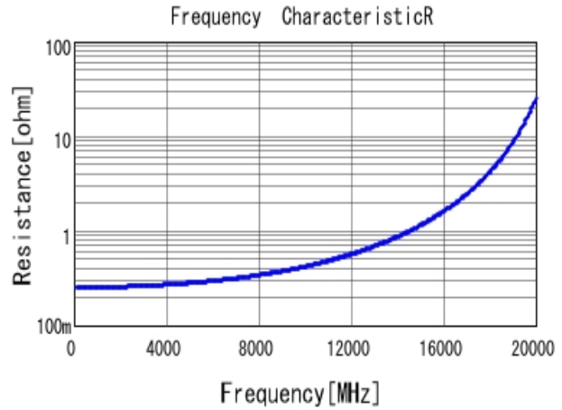
■ GJM1555C1HR90WB01 R DCOV, 25degC
