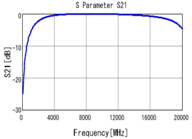
■ GJM1555C1HR90WB01 S21 DCOV, 25degC
