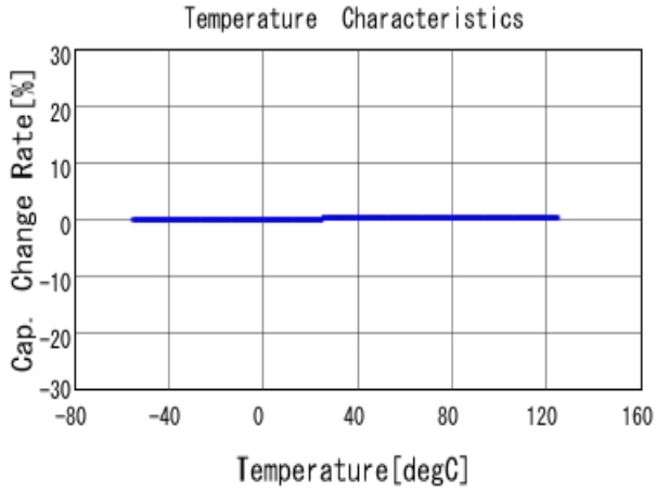
■ GJM1555C1HR90WB01 C-Temp. capchange, DCOV, AC1Vrms
