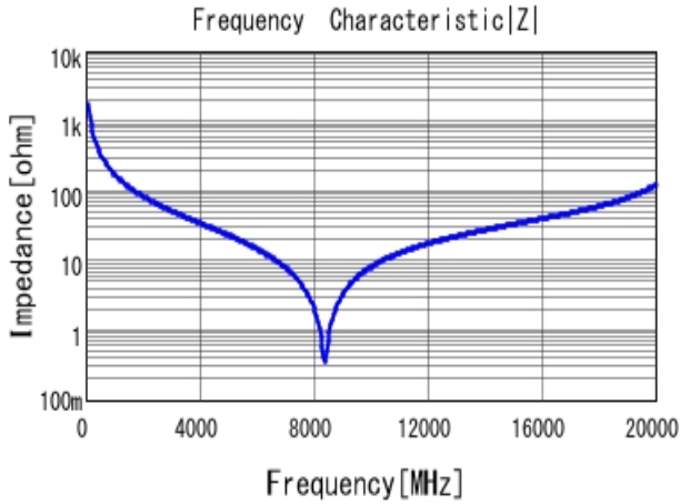
■ GJM1555C1HR90WB01 |Z| DCOV, 25degC
