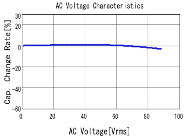
■ GCJ31BR72E223KXJ1 C-AC Voltage capchange, DCOV, 25.0d
