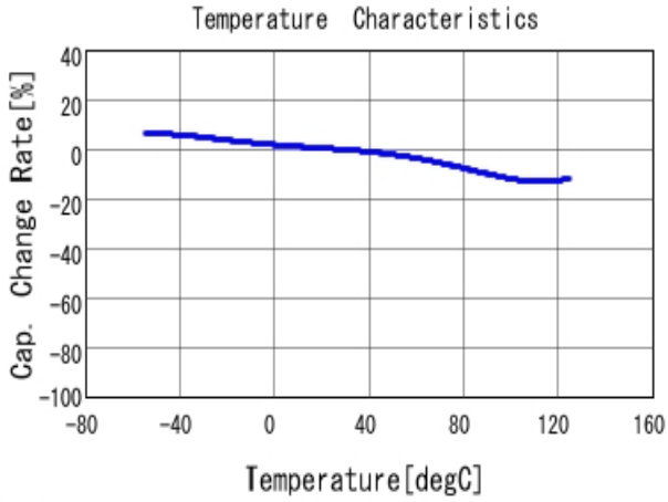
■ GCJ31BR72E223KXJ1 C-Temp. capchange, DCOV, AC1Vrms
