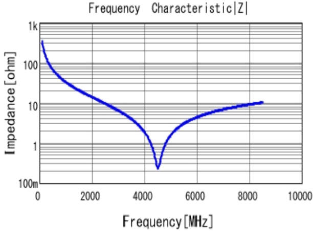
GJM0335C1E4R6BB01 |Z| DC0V, 25degC
