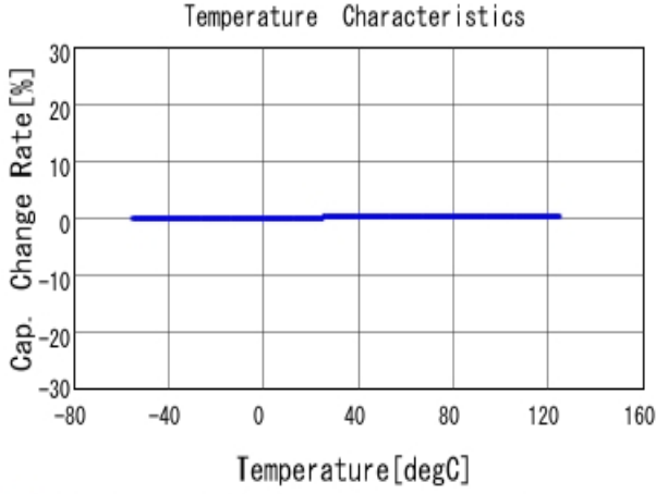
■ GJM0335C1E4R6BB01 C-Temp. capchange, DCOV, AC1Vrms
