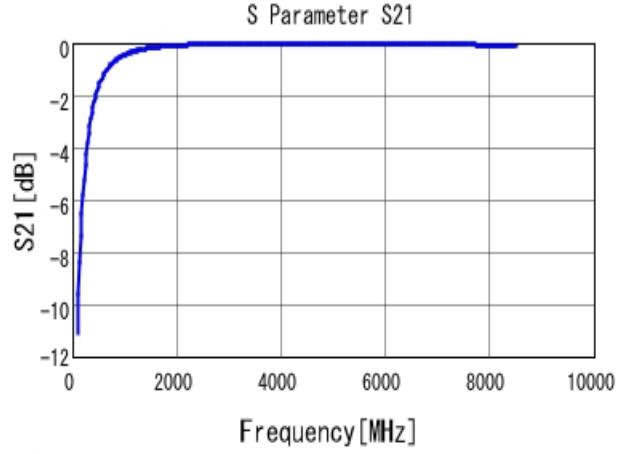
■ GJM0335C1E4R6BB01 S21 DCOV, 25degC
