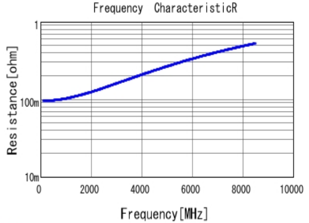
GJM0335C1E4R6BB01 R DC0V, 25degC
