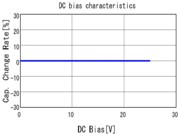
GJM0335C1E4R6BB01 C-DC bias capchange, 25.0degC, AC1V
