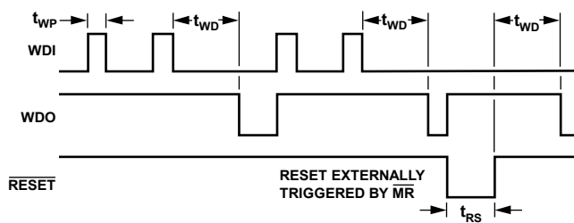
Figure 16. Watchdog Timing
