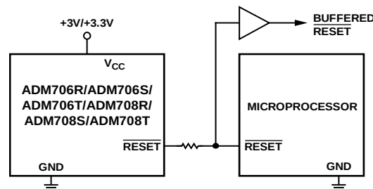
Figure 23. Bidirectional Input/Output RESET
