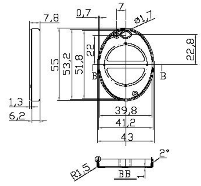
Cover
