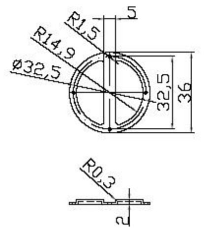
Rubber Button
