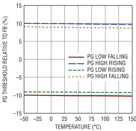
Power-Good Thresholds
