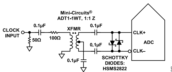
Figure 50. Transformer-Coupled Differential Clock (Up to 200 MHz)
