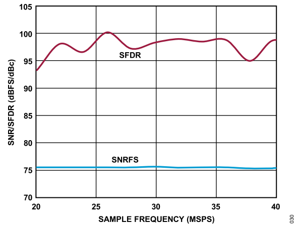
Figure 31. SNR/SFDR vs. Encode, f_{IN} = 30.5 \text{ MHz} , CLK Divider = 4
