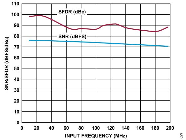
Figure 30. SNR/SFDR vs. f_{IN} , f_{SAMPLE} = 40 \text{ MSPS}
