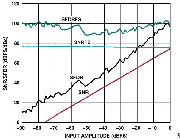
Figure 27. SNR/SFDR vs. Analog Input Level, f_{IN} = 9.7 \text{ MHz} , f_{SAMPLE} = 40 \text{ MSPS}
