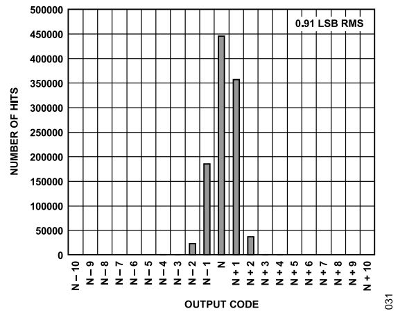
Figure 32. Input-Referred Noise Histogram, f_{SAMPLE} = 40 \text{ MSPS}
