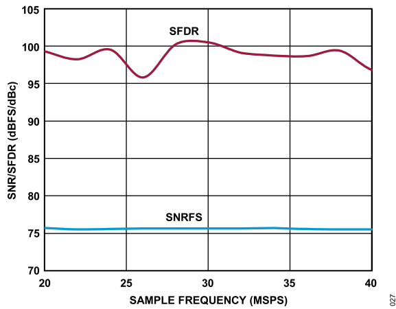
Figure 28. SNR/SFDR vs. Encode, f_{IN} = 19.7 \text{ MHz} , CLK Divider = 4
