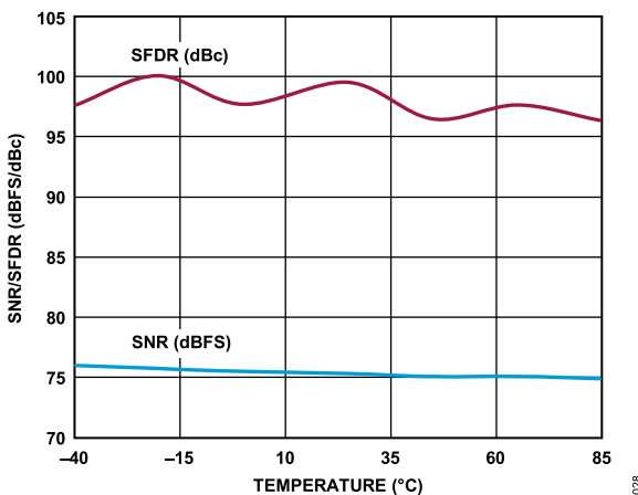
Figure 29. SNR/SFDR vs. Temperature, f_{IN} = 9.7 \text{ MHz} , f_{SAMPLE} = 40 \text{ MSPS}
