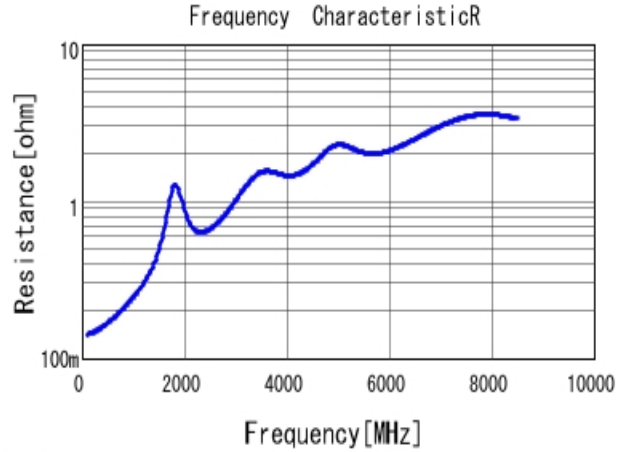
■ GRM1885C2A680JA01 R DCOV, 25degC
