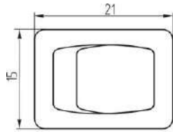
Outline Drawing
