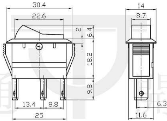
Outline Drawing
