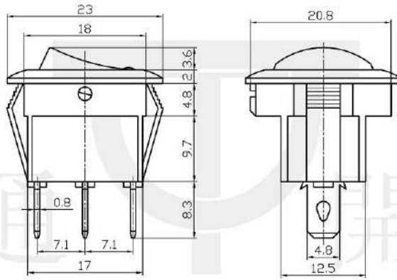
Outline Drawing
