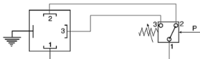
Electrical Connection
