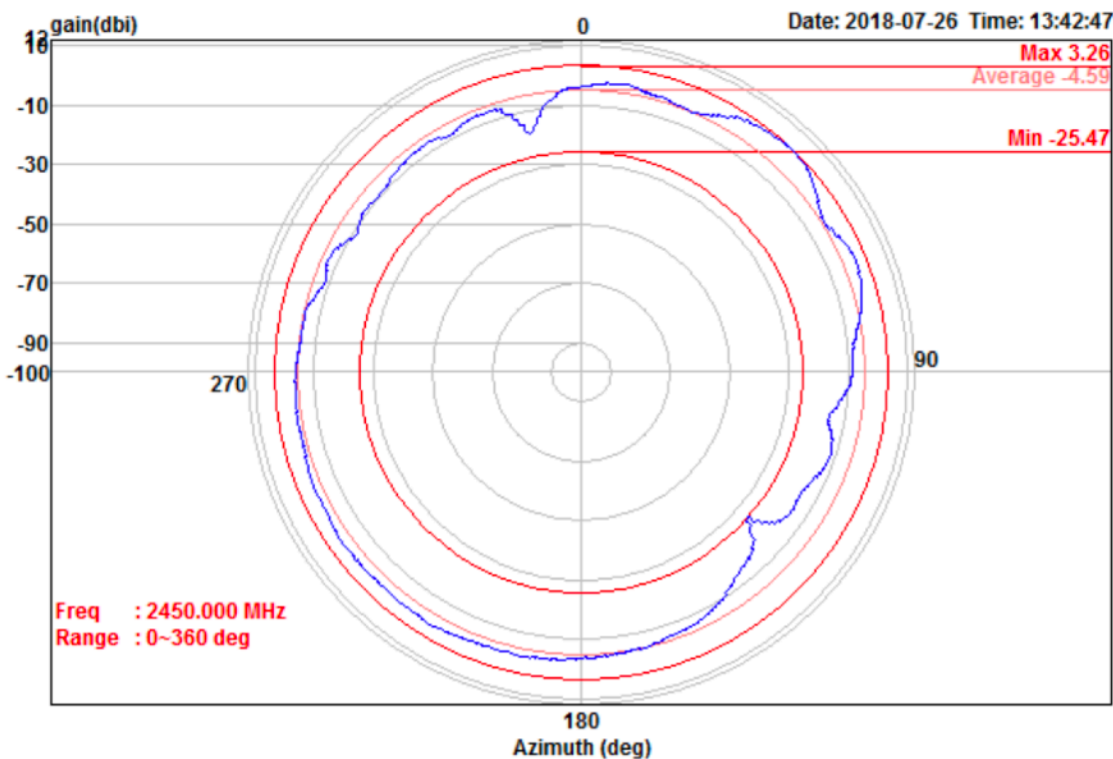
ANT020 Radiation pattern
