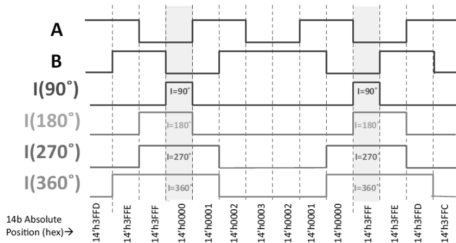
Figure 3: ABI Signal (4096 CPR, with Different I-Width Settings), Assuming the User Sets Hysteresis at 0.02 Mechanical Degrees
