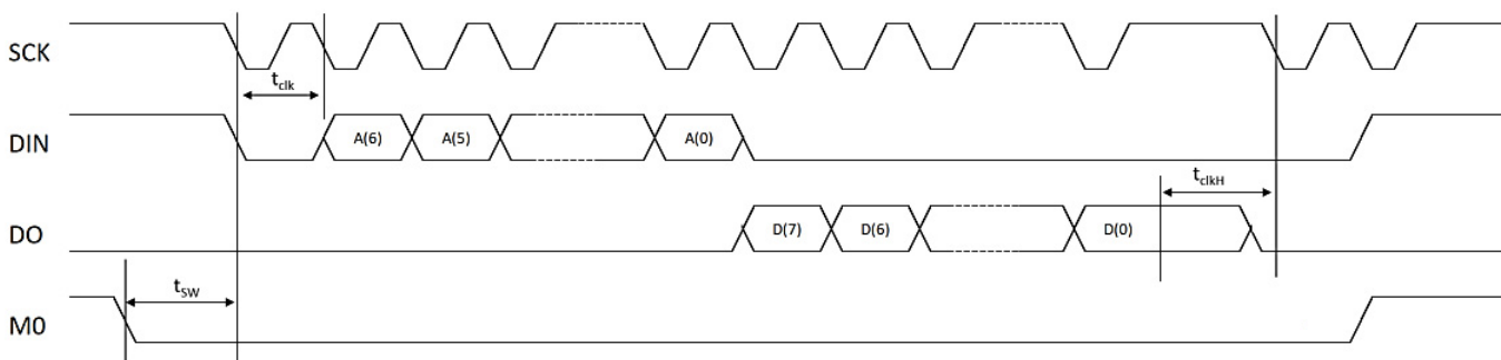
SPI3 Timing Diagram
