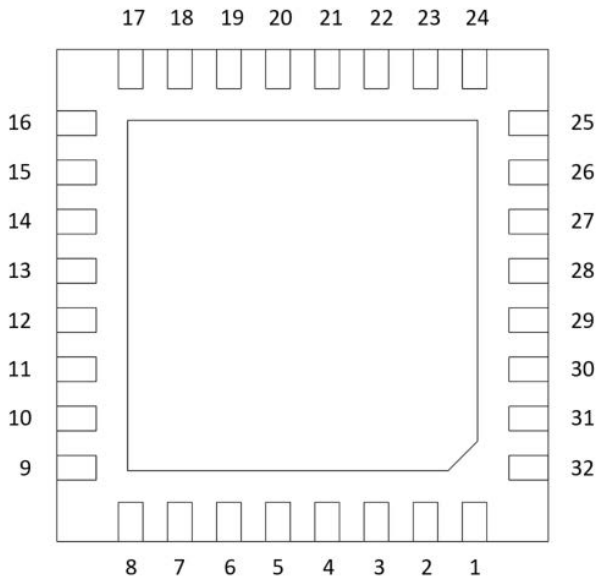
Figure 2: Pin Configurations
