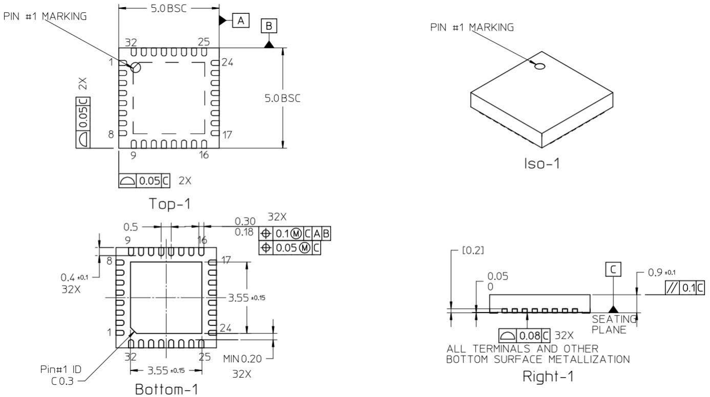
Figure 5: AEAT-9955, 32 QFN Dimensions
