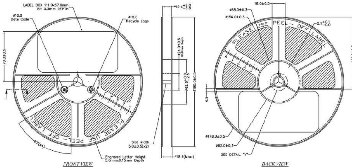
Figure 6: Reel Dimensions
