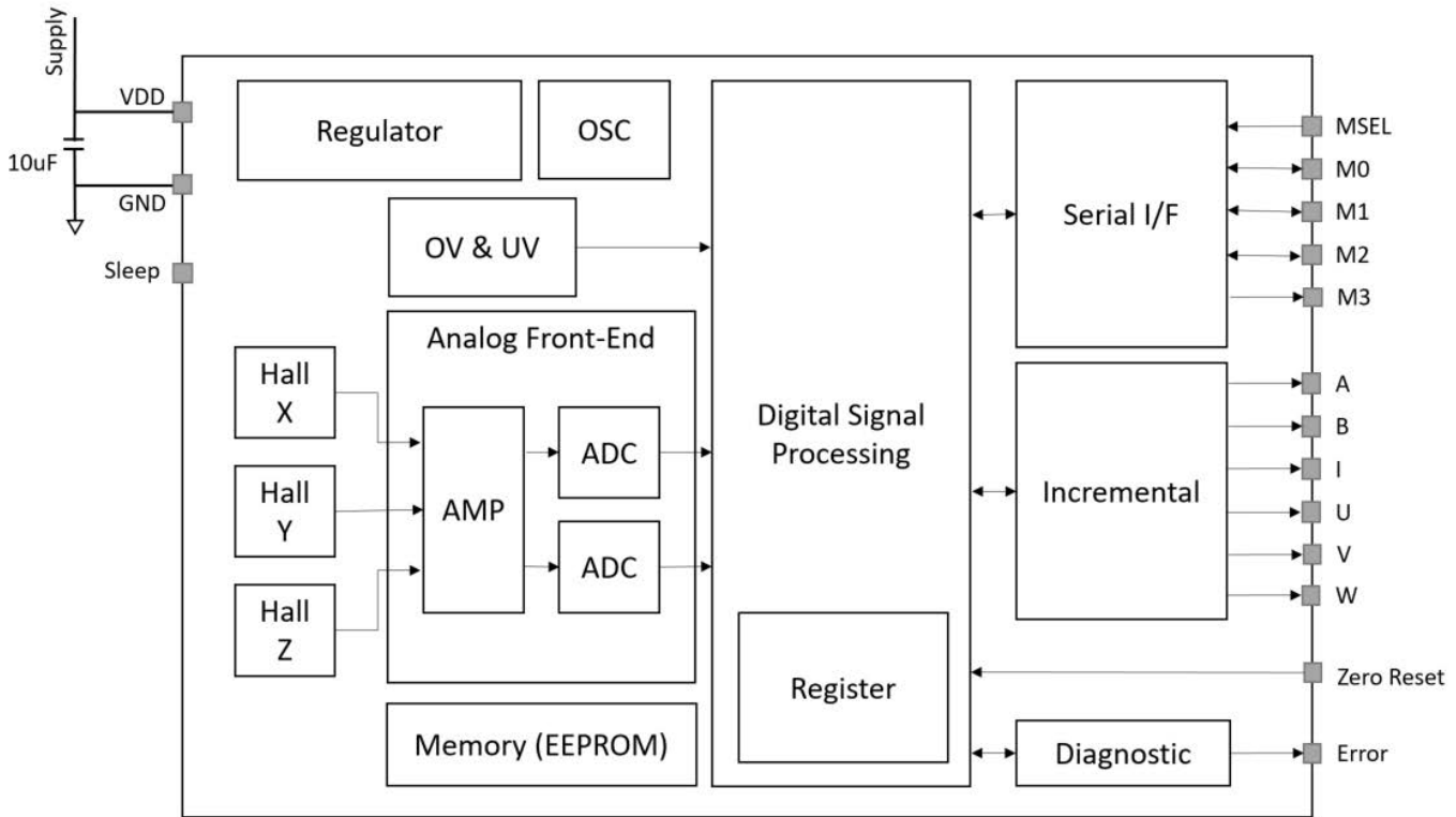
Figure 1: AEAT-9955 Block Diagram
