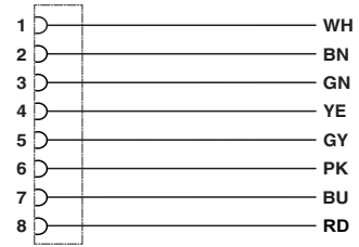
Contact assignment of M8 socket
