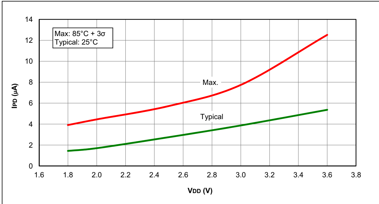
FIGURE 31-39: I_{PD} , TIMER1 OSCILLATOR, F_{osc} = 32 kHz, PIC16LF1938/9 ONLY
