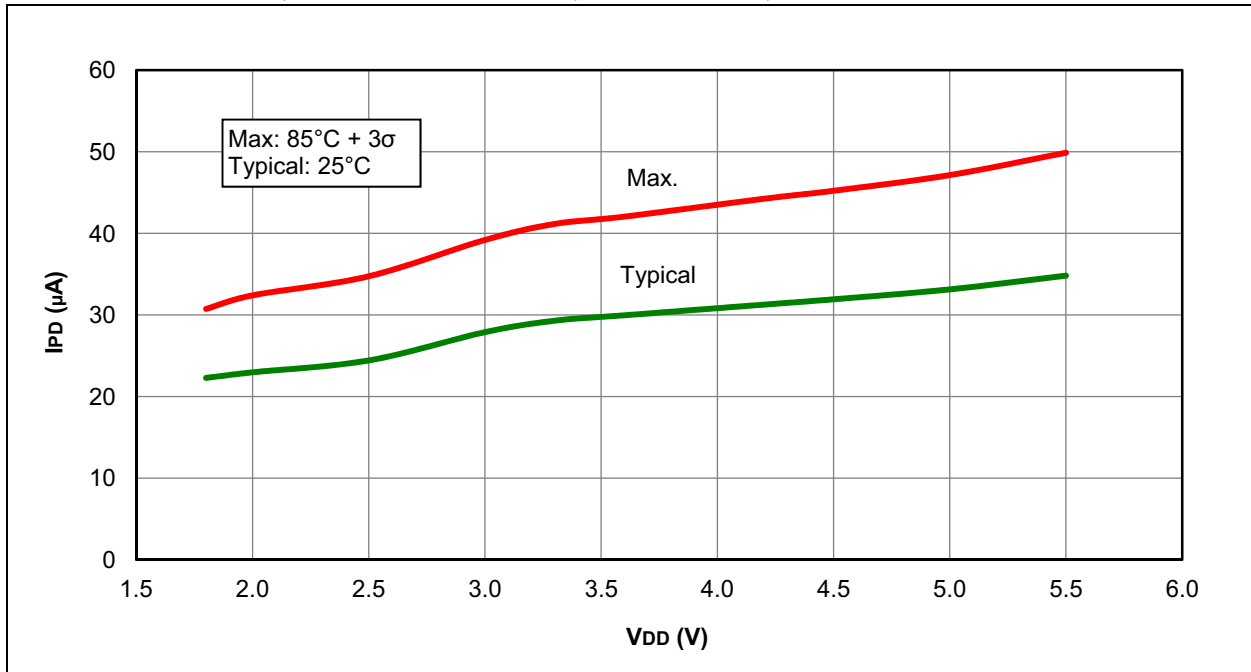
FIGURE 31-40: I_{PD} , TIMER1 OSCILLATOR, F_{osc} = 32 kHz, PIC16F1938/9 ONLY
