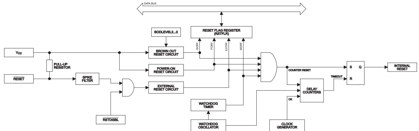
Figure 8-1. Reset Logic
