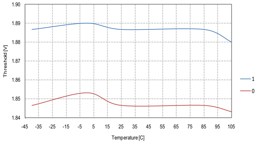
Figure 26-67. BOD Threshold vs. Temperature, BOD Level = 1.8V
