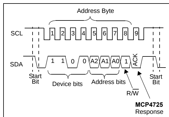
FIGURE 8-2: I 2 C Bus Connection Test.
