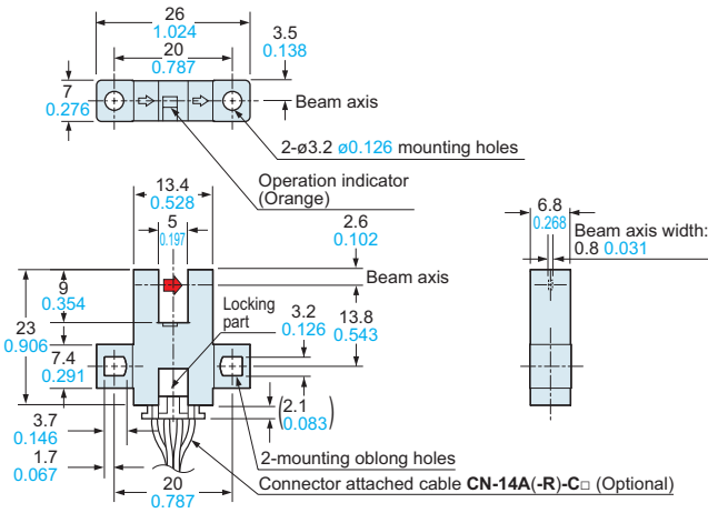
PM-K64(P) Sensor
