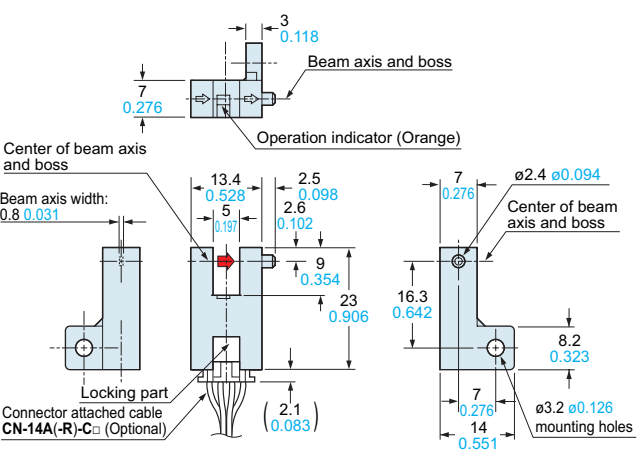
PM-F64(P) Sensor
