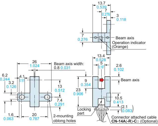
PM-L64(P) Sensor
