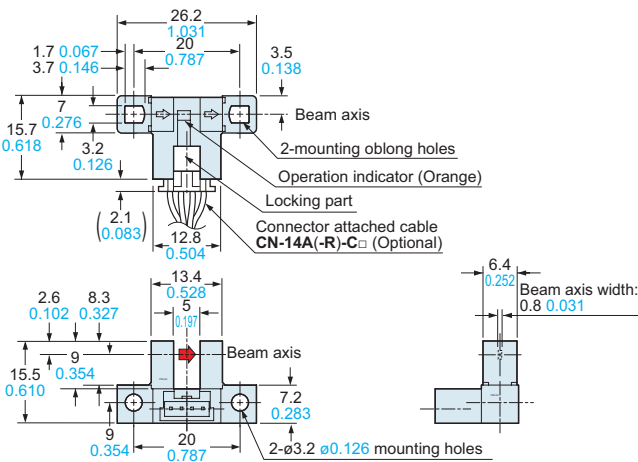
PM-L64(P) Sensor
