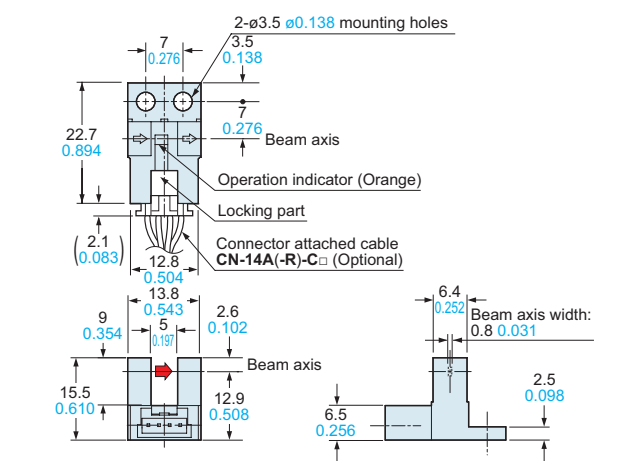
PM-Y64(P) Sensor
