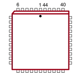
44-Lead PLCC (PJ) (top view)
