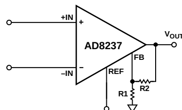
Figure 70. Applying Gain to the Reference Voltage
