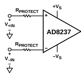
Figure 68. Protection Resistors for Large Input Voltages
