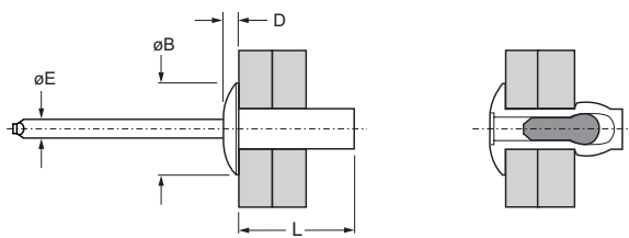
AD H / AD SB Dome head Tête bombée / Flachrundkopf / Testa tonda / Cabeza alomada
