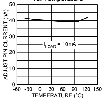
MIC29302/3 Adjust Pin Current vs. Temperature
