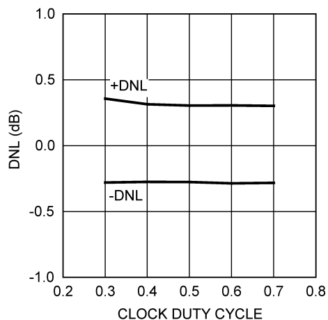
Figure 6. DNL vs. Clock Duty Cycle (DC input)
