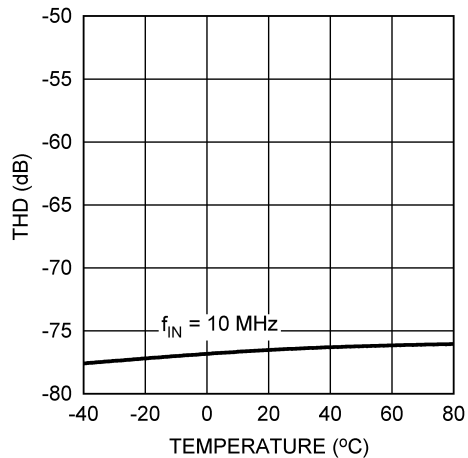
Figure 26. THD vs. Temperature
