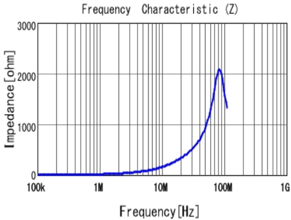
LQM21PN2R2NGC |Z|
