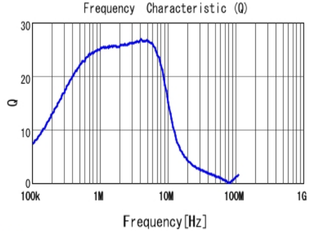
LQM21PN2R2NGC Q
