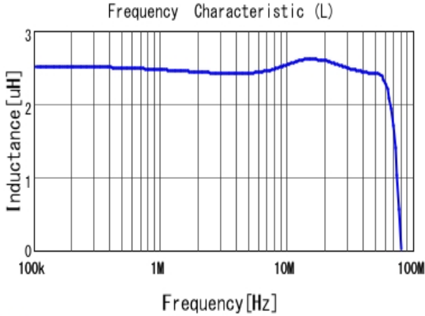
LQM21PN2R2NGC L
