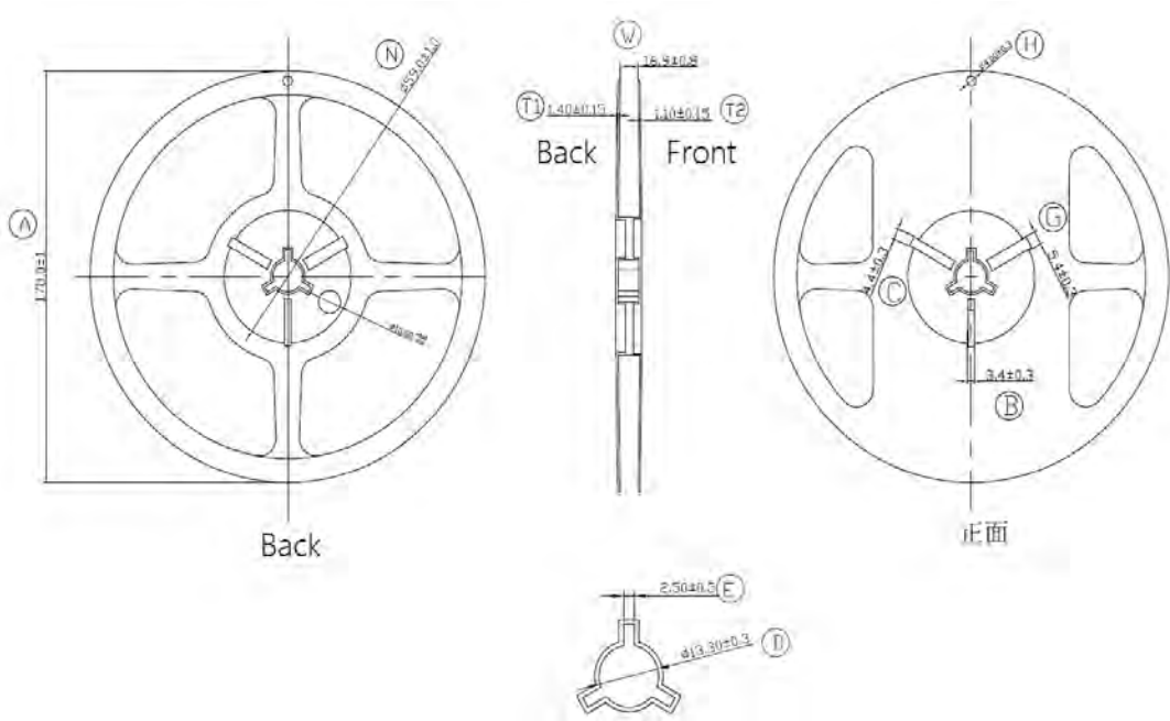
Figure 12. Reel dimensions for LUXEON 7070.
