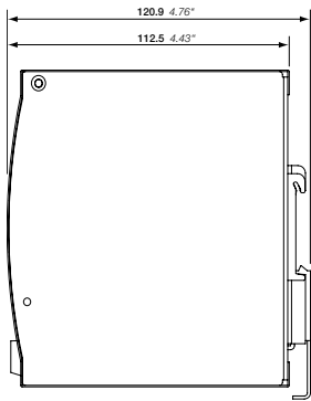
CP-T 24/40.0, CP-T 48/20.0
