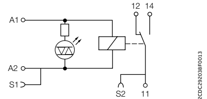
RB(R)121-12VDC/24VDC
