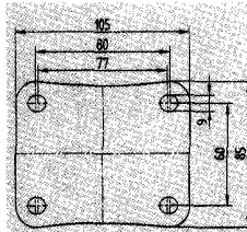
Swivel Castor P62-105x85
