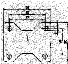
Fixed Castor P62-103x85
