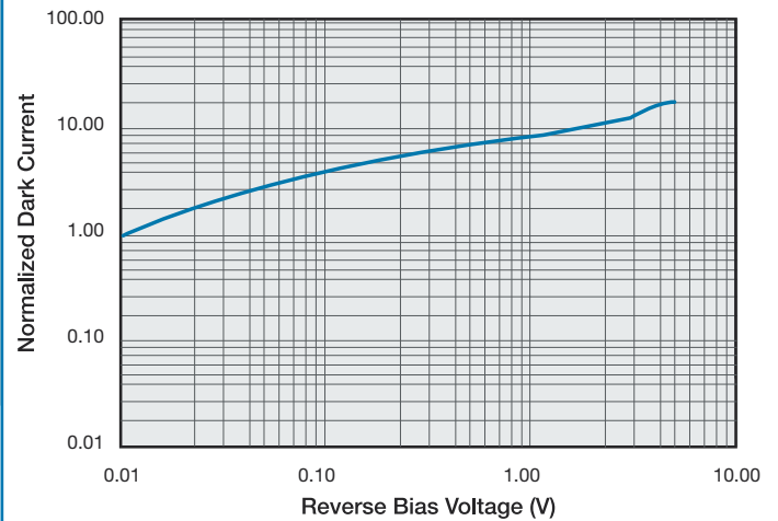
■ Typ. Dark Current vs. Reverse Bias ( T_A = 25^\circ\text{C} , Normalized at -0.01\text{V} )
